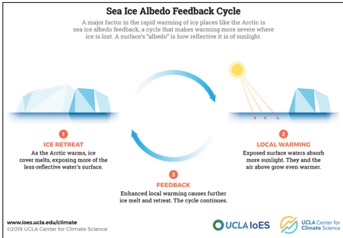
Figure 2. Sea ice albedo feedback cycle (Graphic: UCLA Center for Climate Science, courtesy of Alex Hall).
