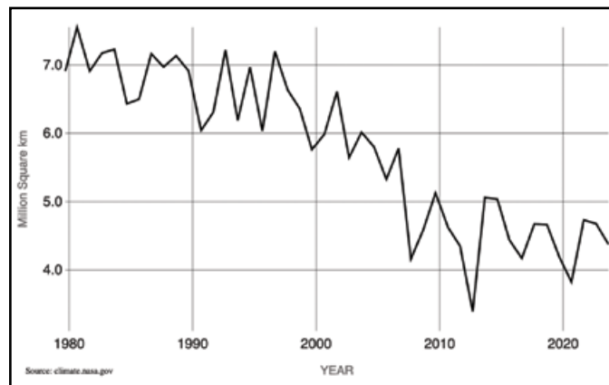
Figure 3. Annual September minimum extent in sea ice since 1979 from satellite observations (Source: NASA; https://climate.nasa.gov/vital-signs-hds/arctic-sea-ice/ ).
